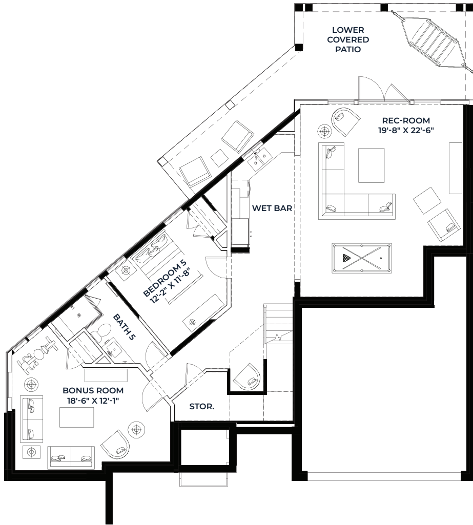
LOWER FLOOR
