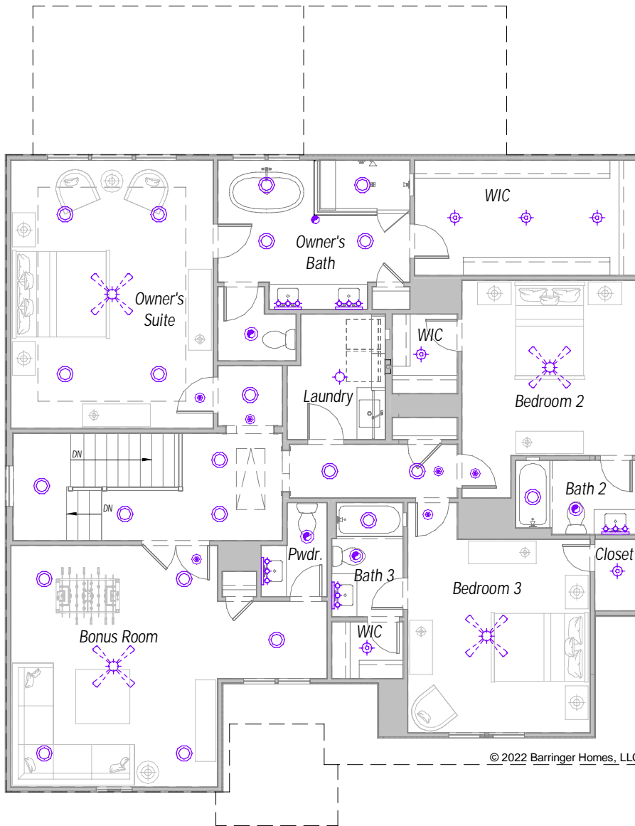
Upper Level Electrical
