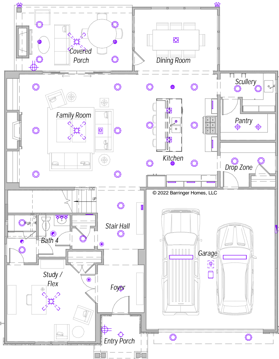
Main Level - Electrical
