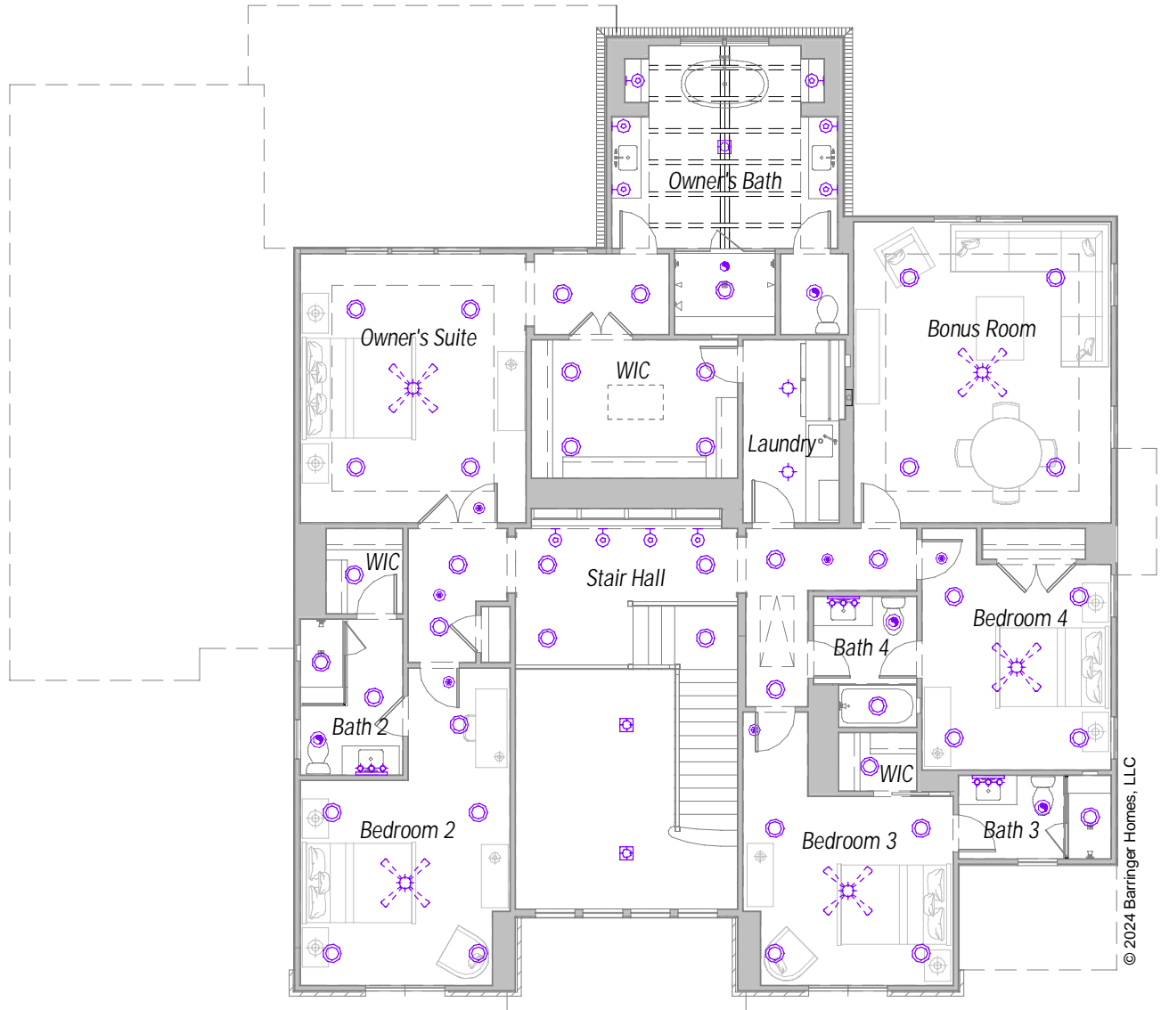
Upper Level Electrical
